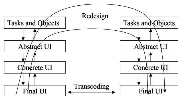
Figure 4. Approaches to changing the design for a different platform.
