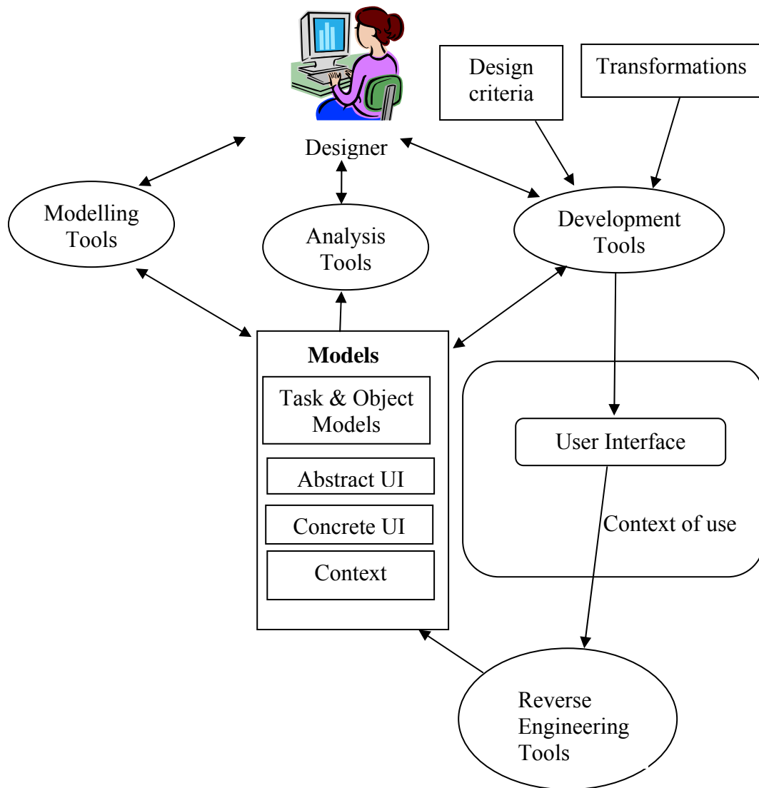
Figure 1: Models and Related Tools in the User Interface Development Process.
