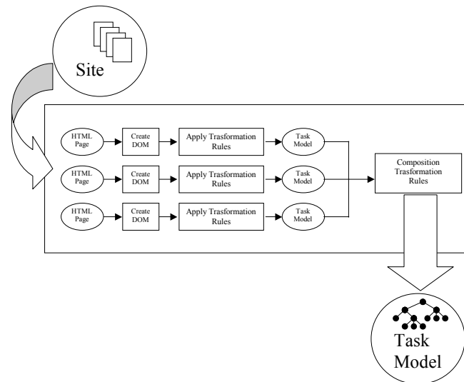
Figure 3. The architecture of WebRevEnge.
