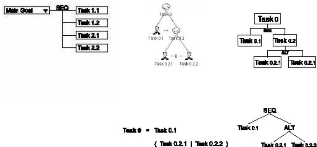
Figure 2: Graphical notations for task modelling.
